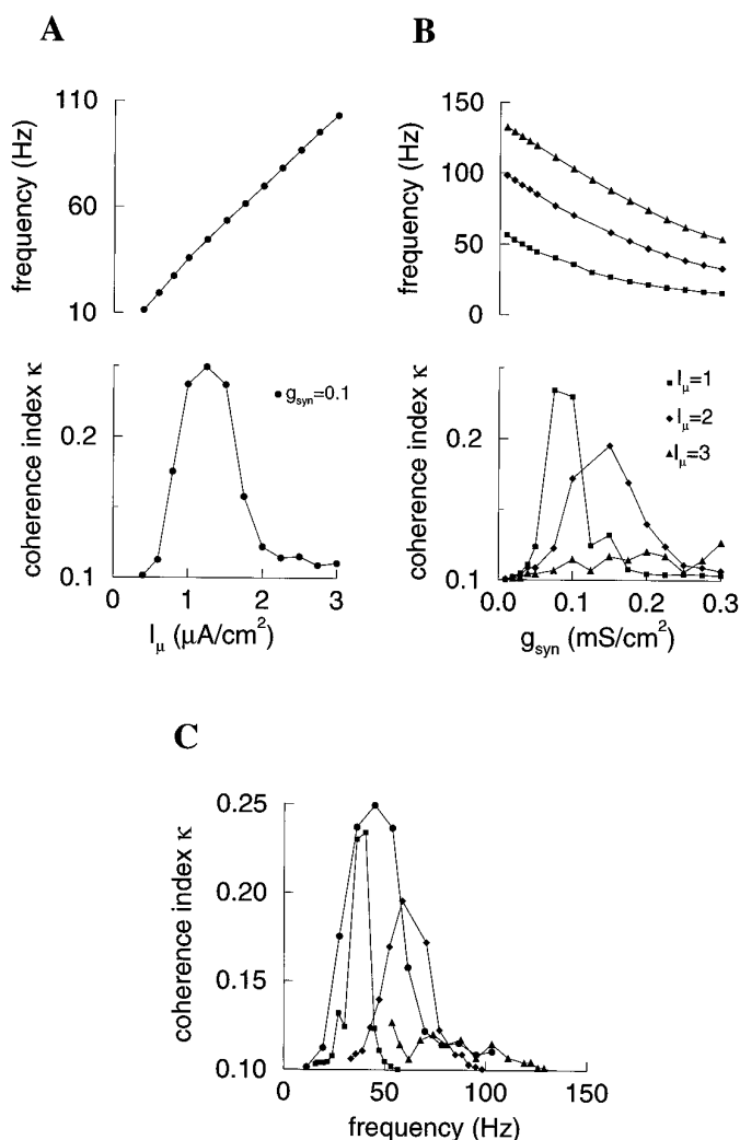
Figure 12. High network coherence in the gamma oscillation frequency range. A , With increasing mean drive I_{\mu} , the average oscillation frequency monotonically increases (top), but the coherence index \kappa is large only for intermediate I_{\mu} values (bottom). B , Similarly, as the maximal synaptic conductance g_{\text{syn}} is increased, with stronger inhibitory interactions the average oscillation frequency f_{\mu} monotonically decreases (top). An increase in the external drive shifts the curve upwards. On the other hand, the coherence index \kappa displays a pronounced peak for I_{\mu} = 1 , which flattens for larger I_{\mu} values (bottom). C , The coherence index is plotted as function of f_{\mu} for all four curves from ( A , B ). The macroscopic network coherence is observed only in the gamma range of the oscillation frequencies (20–80 Hz) ( M_{\text{syn}} = 60 , I_{\sigma} = 0.03 ; the coherence index \kappa was calculated with \tau = 0.1/f_{\mu} ).
